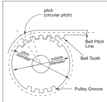
Figure 1 Pulley Dimensions
