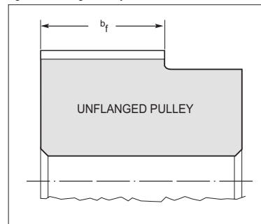
Figure 3 Unflanged Pulley
